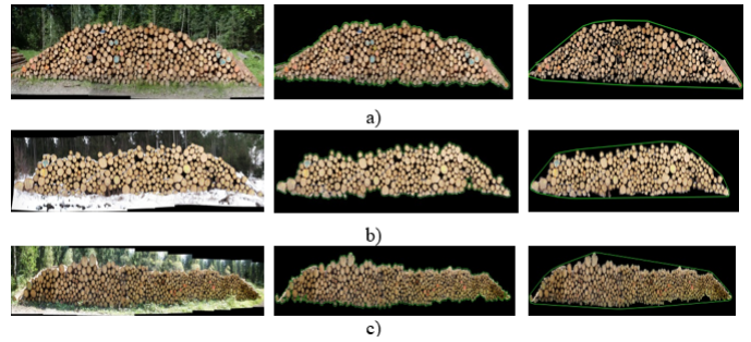
Fig. 8: : Wood stacks detection results 8a) soil, 8b) snow, 8c) grassy area
